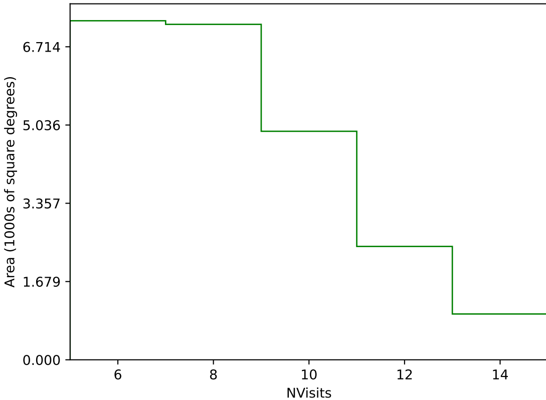
too_elab_r32_d2_ugrizy_v3.4_10yrs Yr 1 g band: NVisits
