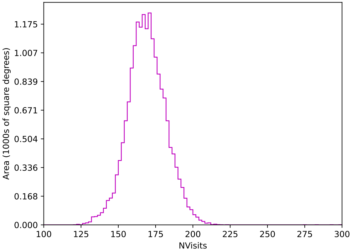
too_elab_r32_d2_ugrizy_v3.4_10yrs WFD z band: NVisits
