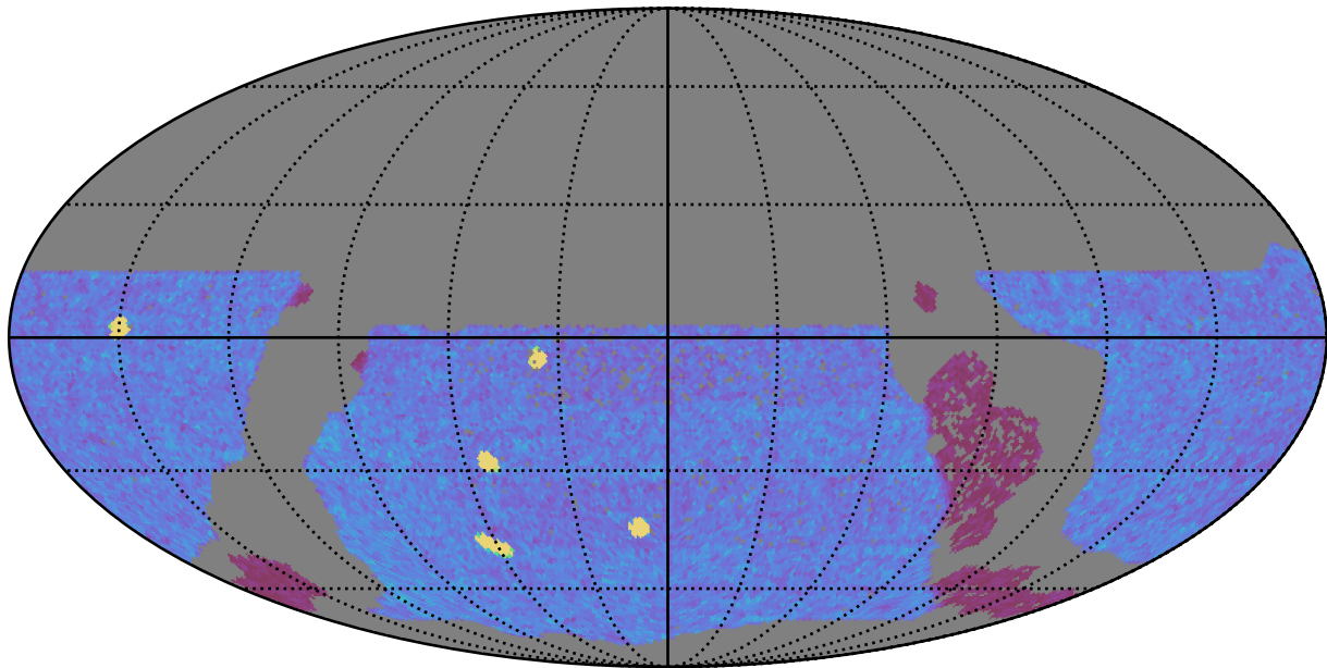
too_elab_r32_d2_ugrizy_v3.4_10yrs WFD y band: NVisits
