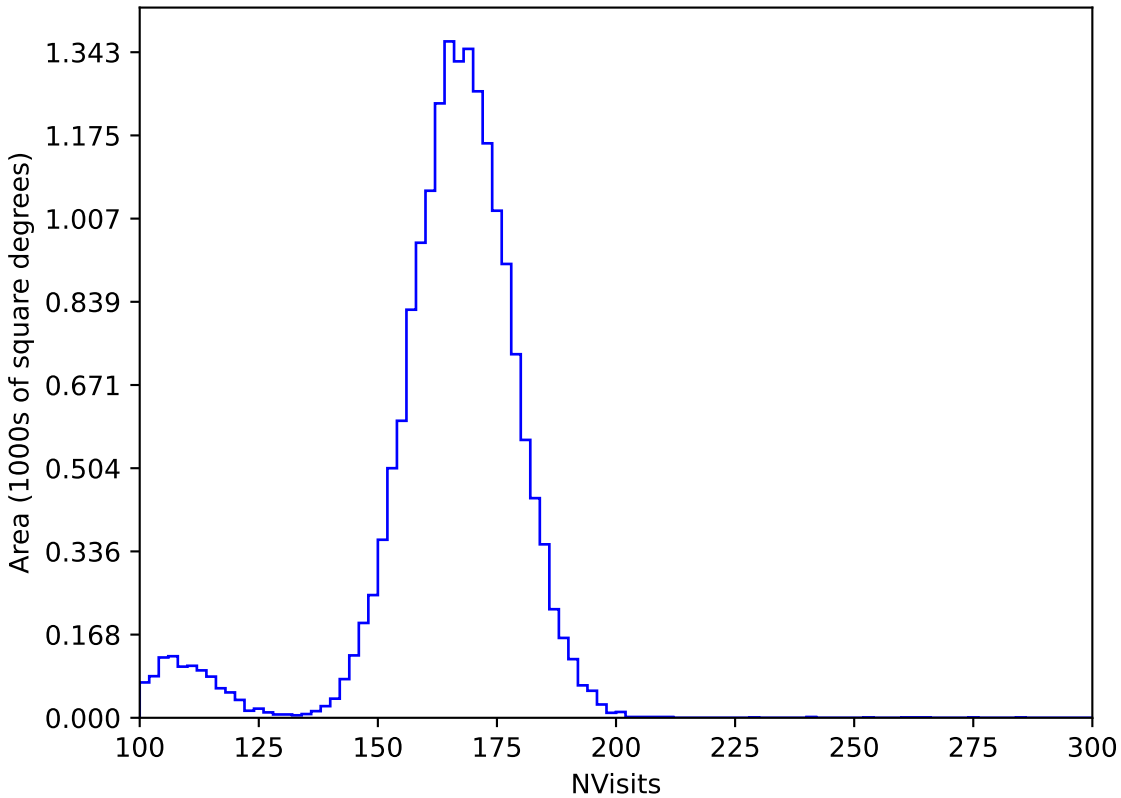
too_elab_r32_d2_ugrizy_v3.4_10yrs WFD y band: NVisits
