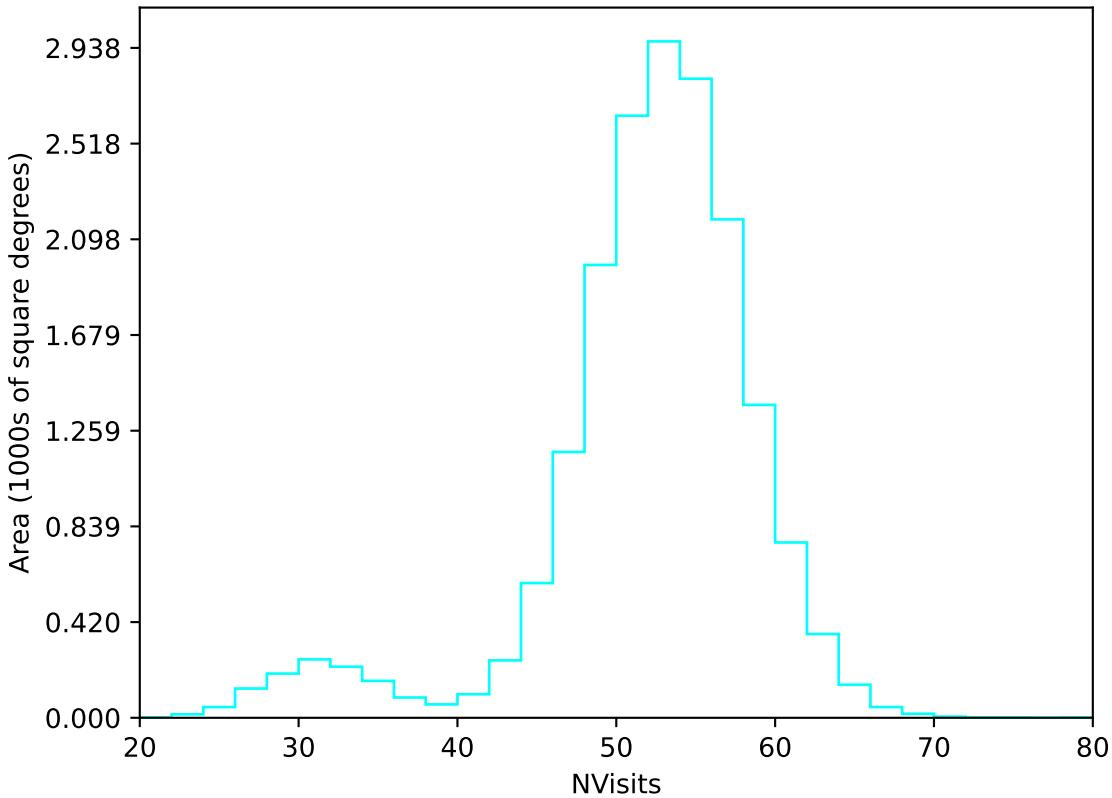
too_elab_r32_d2_ugrizy_v3.4_10yrs WFD u band: NVisits
