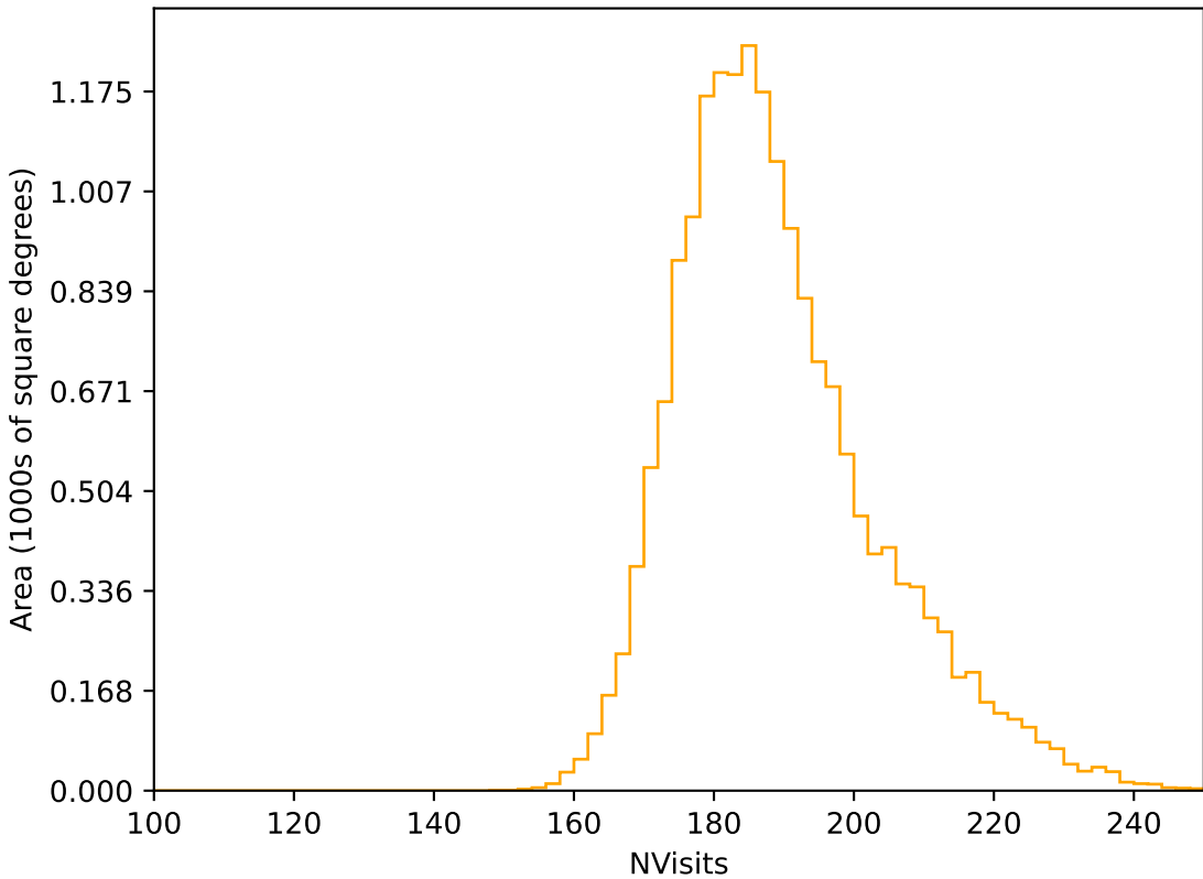
too_elab_r32_d2_ugrizy_v3.4_10yrs WFD r band: NVisits
