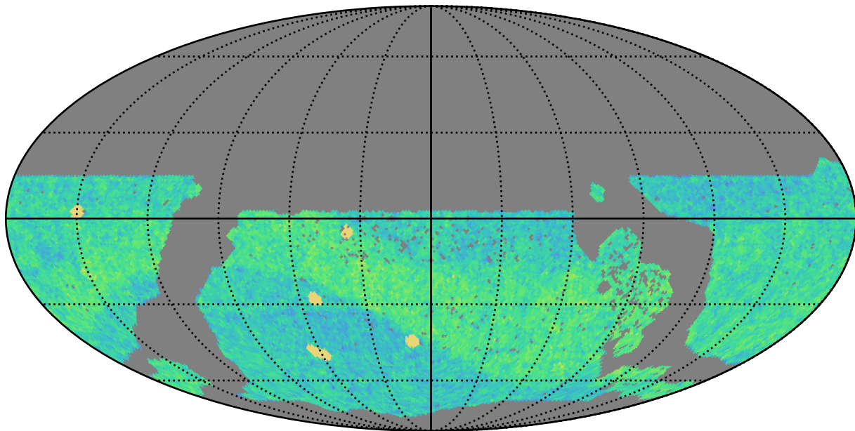
too_elab_r32_d2_ugrizy_v3.4_10yrs WFD i band: NVisits
