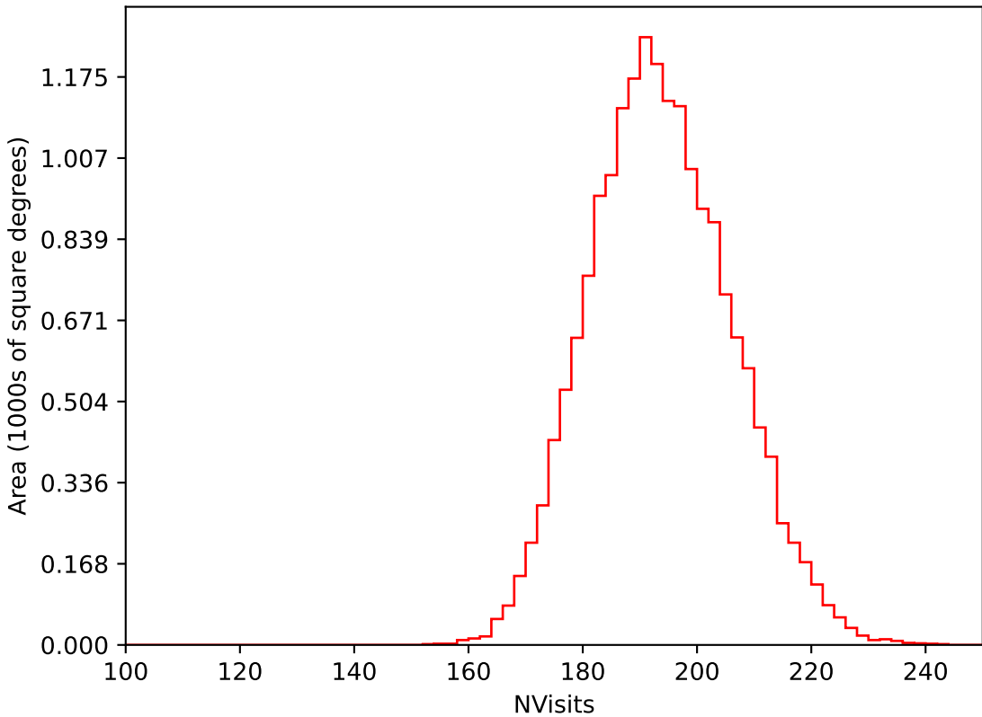
too_elab_r32_d2_ugrizy_v3.4_10yrs WFD i band: NVisits
