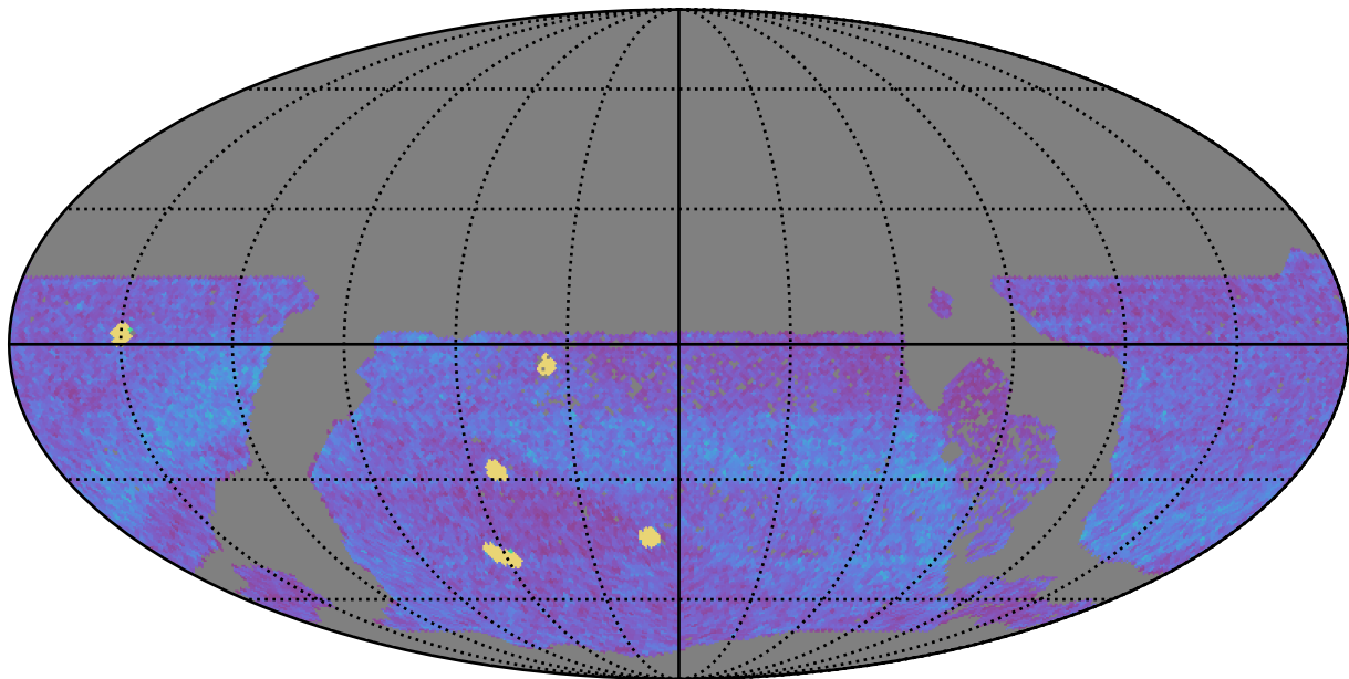
too_elab_r32_d2_ugrizy_v3.4_10yrs WFD all bands: NVisits
