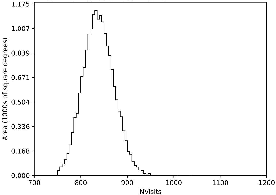
too_elab_r32_d2_ugrizy_v3.4_10yrs WFD all bands: NVisits
