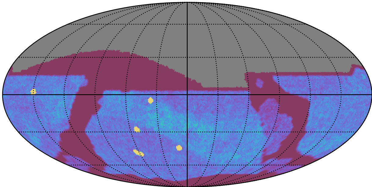
too_elab_r32_d2_ugrizy_v3.4_10yrs All sky z band: NVisits
