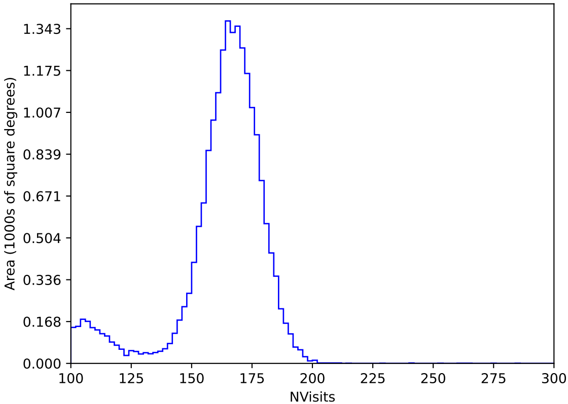
too_elab_r32_d2_ugrizy_v3.4_10yrs All sky y band: NVisits
