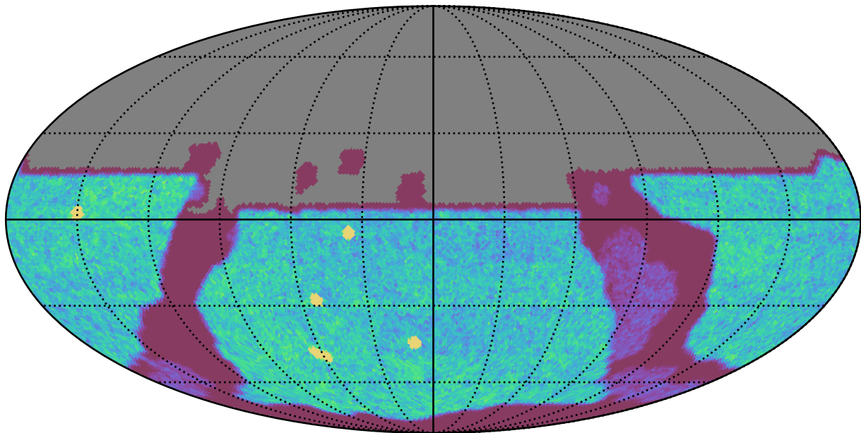
too_elab_r32_d2_ugrizy_v3.4_10yrs All sky u band: NVisits
