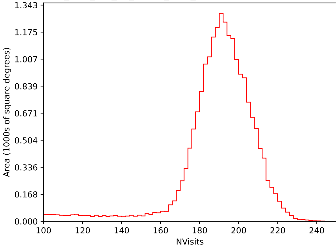
too_elab_r32_d2_ugrizy_v3.4_10yrs All sky i band: NVisits
