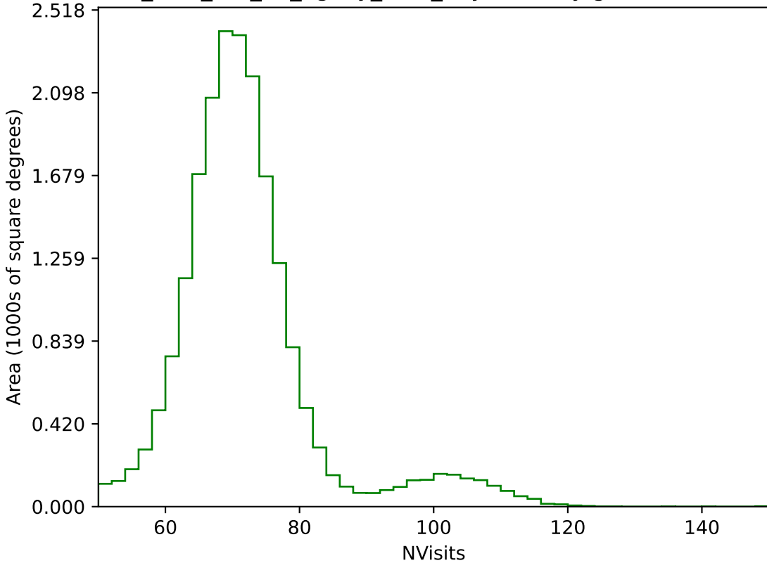
too_elab_r32_d2_ugrizy_v3.4_10yrs All sky g band: NVisits
