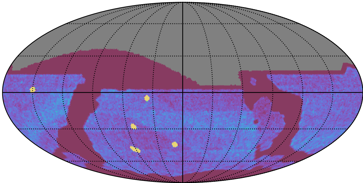
too_elab_r32_d2_ugrizy_v3.4_10yrs All sky all bands: NVisits
