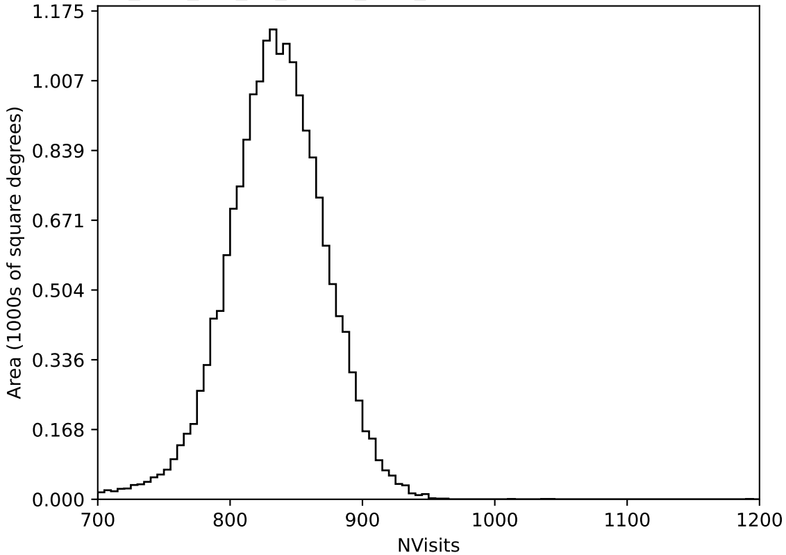
too_elab_r32_d2_ugrizy_v3.4_10yrs All sky all bands: NVisits
