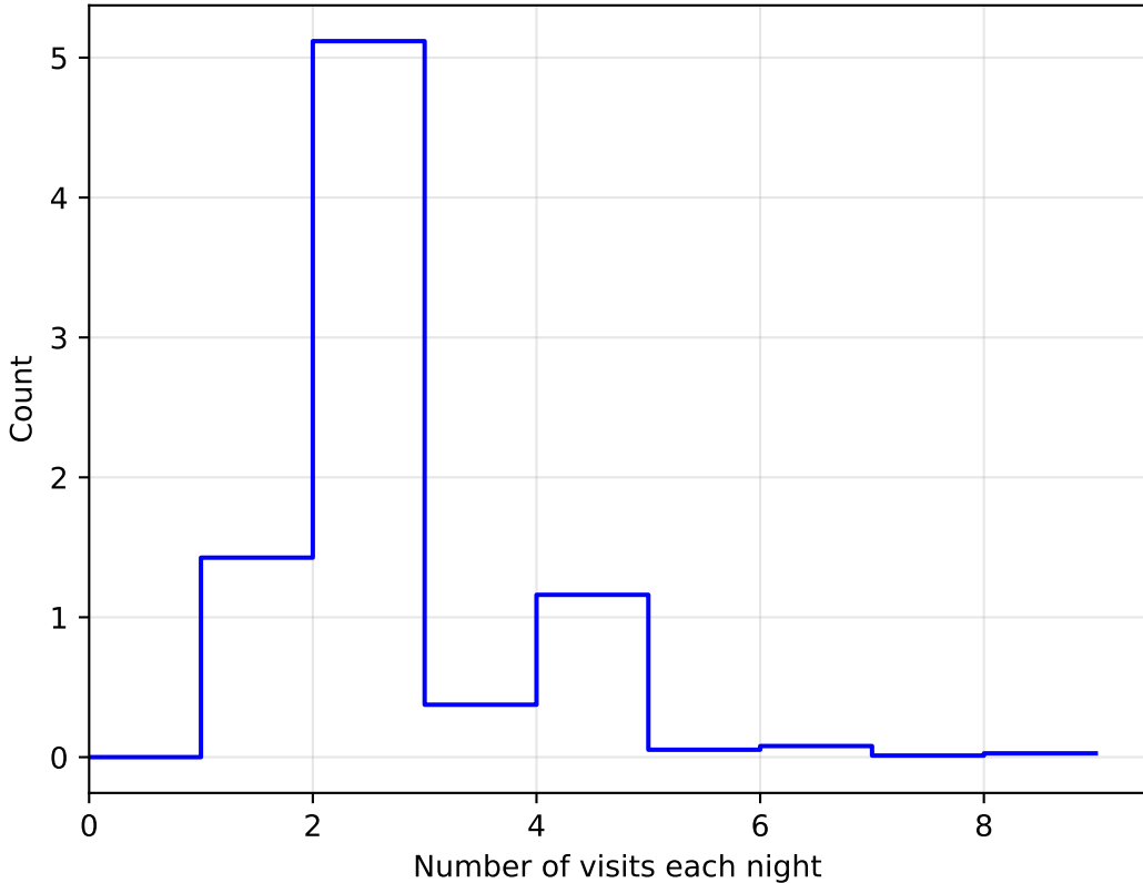
too_elab_r32_d2_ugrizy_v3.4_10yrs WFD: NVisitsPerNight 1e6
