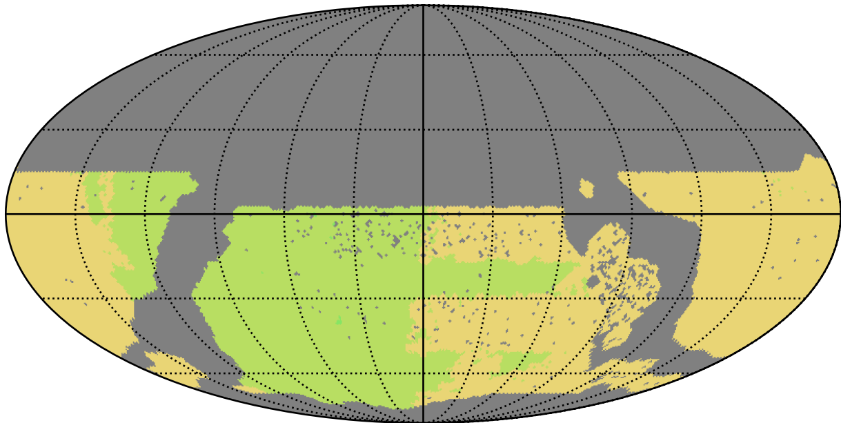
too_elab_r32_d2_ugrizy_v3.4_10yrs WFD all bands: NSeasons
