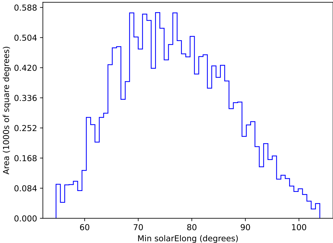
too_elab_r32_d2_ugrizy_v3.4_10yrs WFD u band: Min solarElong
