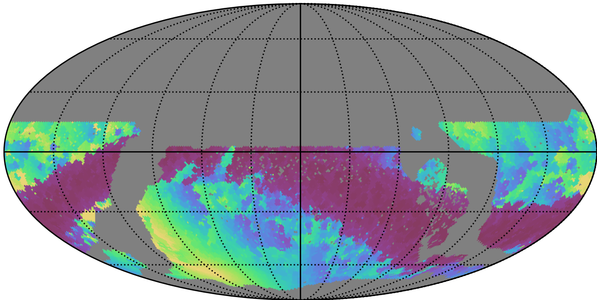
too_elab_r32_d2_ugrizy_v3.4_10yrs WFD r band: Min solarElong
