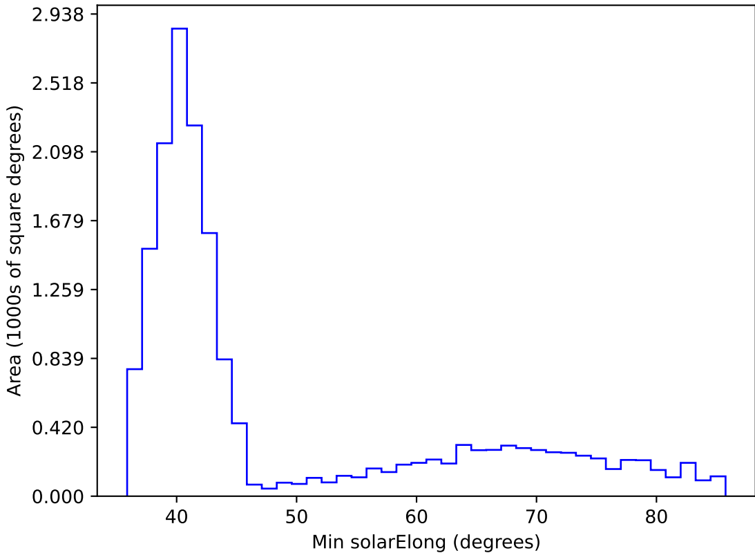
too_elab_r32_d2_ugrizy_v3.4_10yrs WFD i band: Min solarElong
