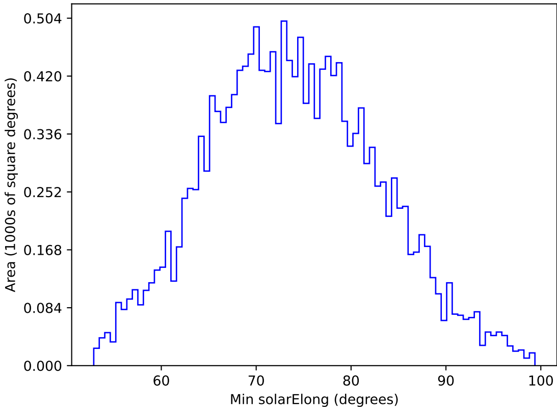
too_elab_r32_d2_ugrizy_v3.4_10yrs WFD g band: Min solarElong
