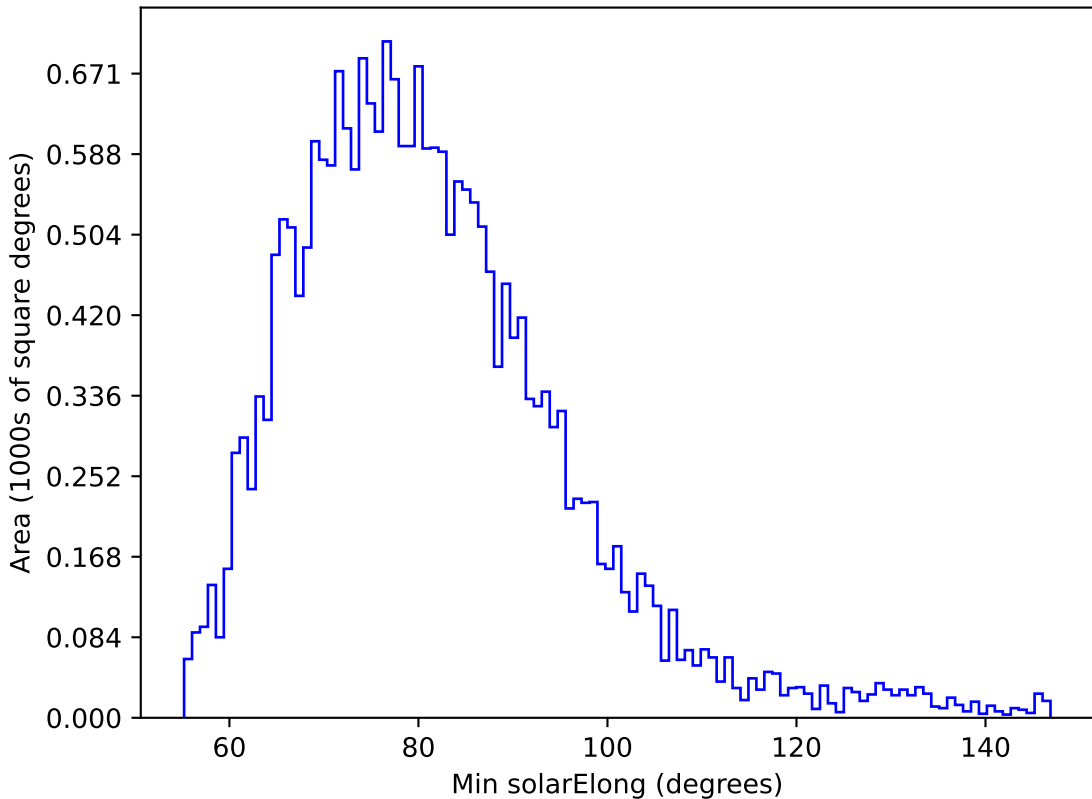
too_elab_r32_d2_ugrizy_v3.4_10yrs All sky u band: Min solarElong
