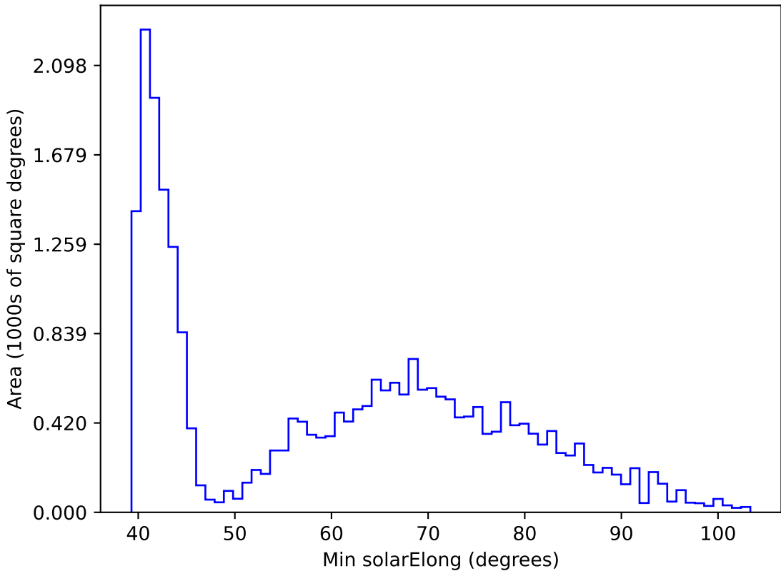
too_elab_r32_d2_ugrizy_v3.4_10yrs All sky r band: Min solarElong
