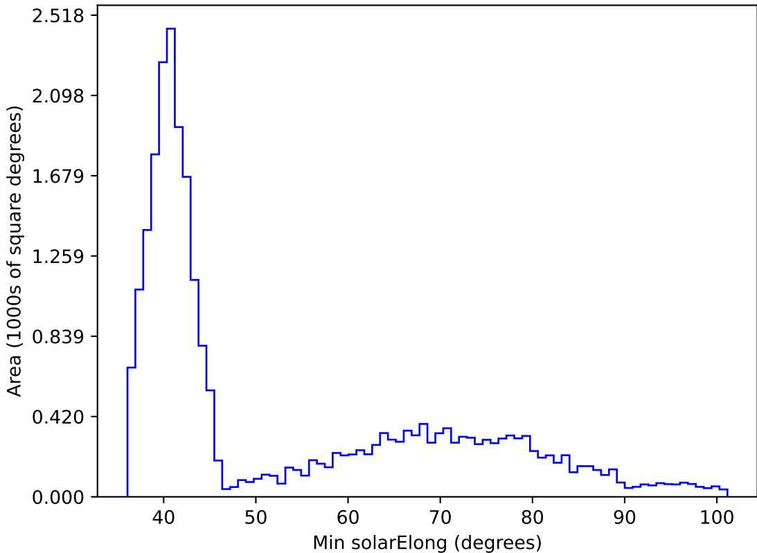
too_elab_r32_d2_ugrizy_v3.4_10yrs All sky i band: Min solarElong
