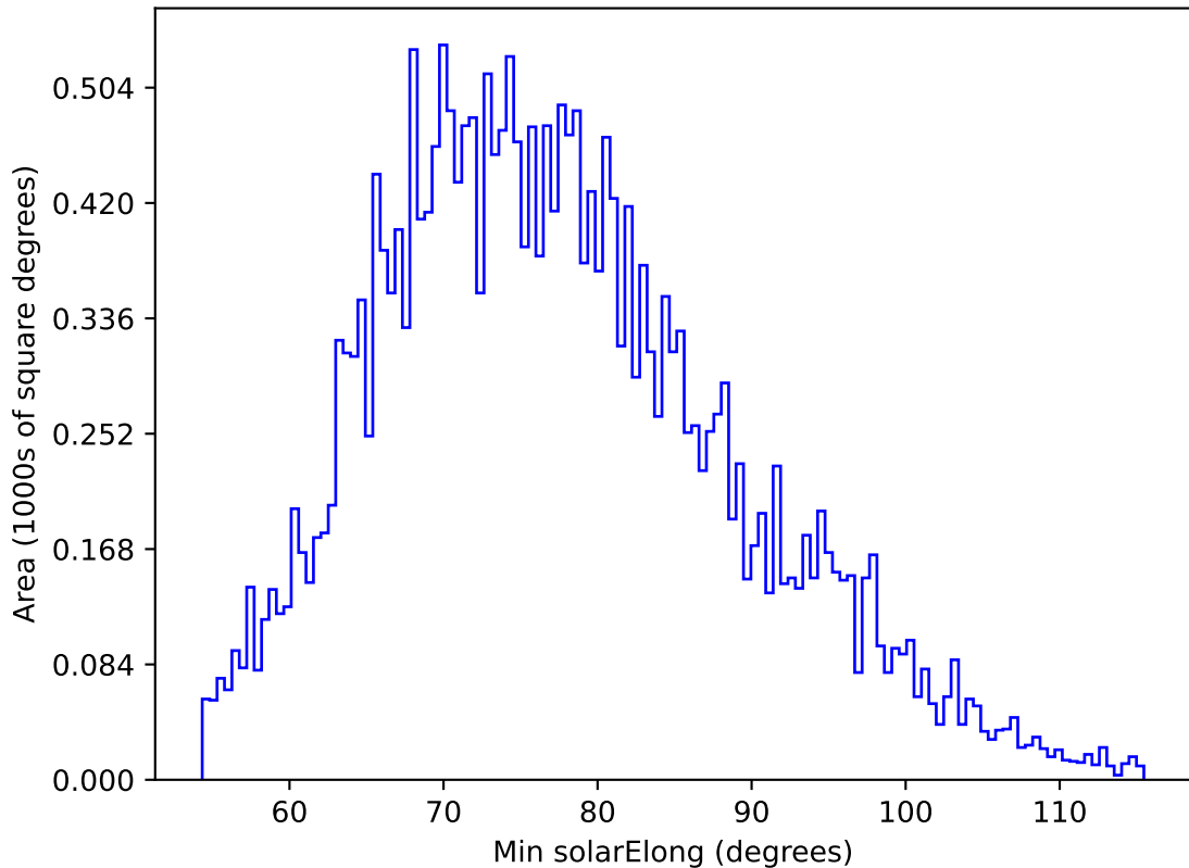
too_elab_r32_d2_ugrizy_v3.4_10yrs All sky g band: Min solarElong
