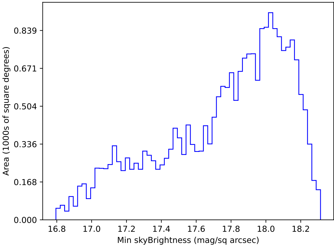
too_elab_r32_d2_ugrizy_v3.4_10yrs Yr 1 y band: Min skyBrightness
