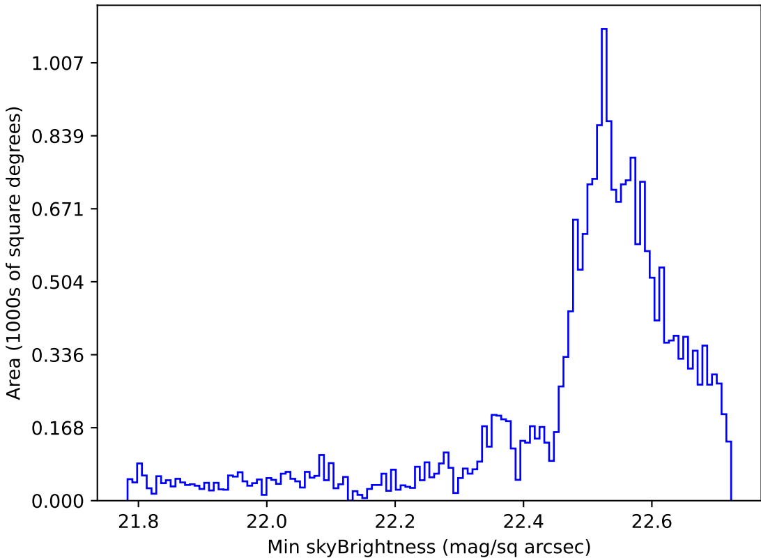
too_elab_r32_d2_ugrizy_v3.4_10yrs Yr 1 u band: Min skyBrightness
