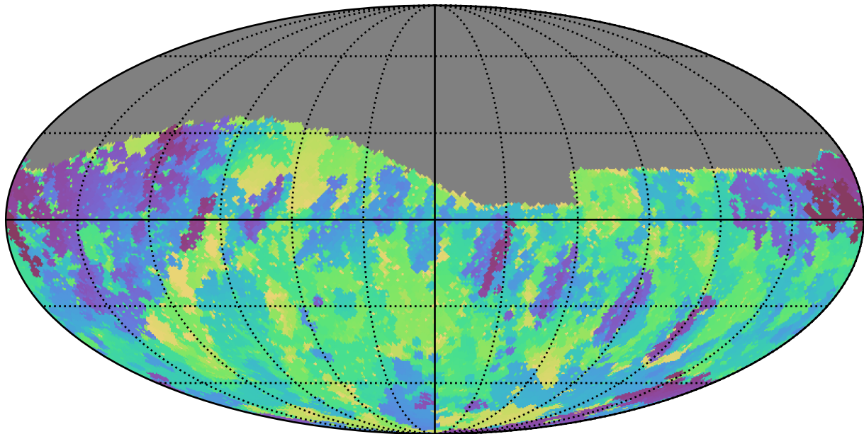
too_elab_r32_d2_ugrizy_v3.4_10yrs Yr 1 r band: Min skyBrightness
