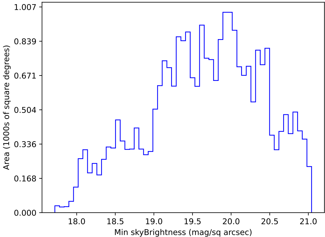
too_elab_r32_d2_ugrizy_v3.4_10yrs Yr 1 r band: Min skyBrightness
