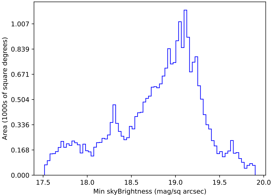
too_elab_r32_d2_ugrizy_v3.4_10yrs Yr 1 i band: Min skyBrightness
