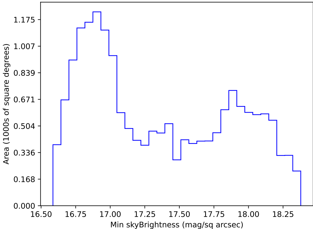
too_elab_r32_d2_ugrizy_v3.4_10yrs WFD z band: Min skyBrightness
