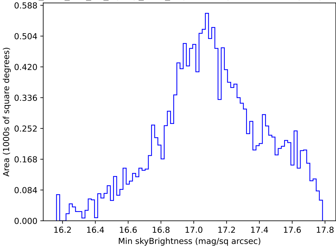
too_elab_r32_d2_ugrizy_v3.4_10yrs WFD y band: Min skyBrightness
