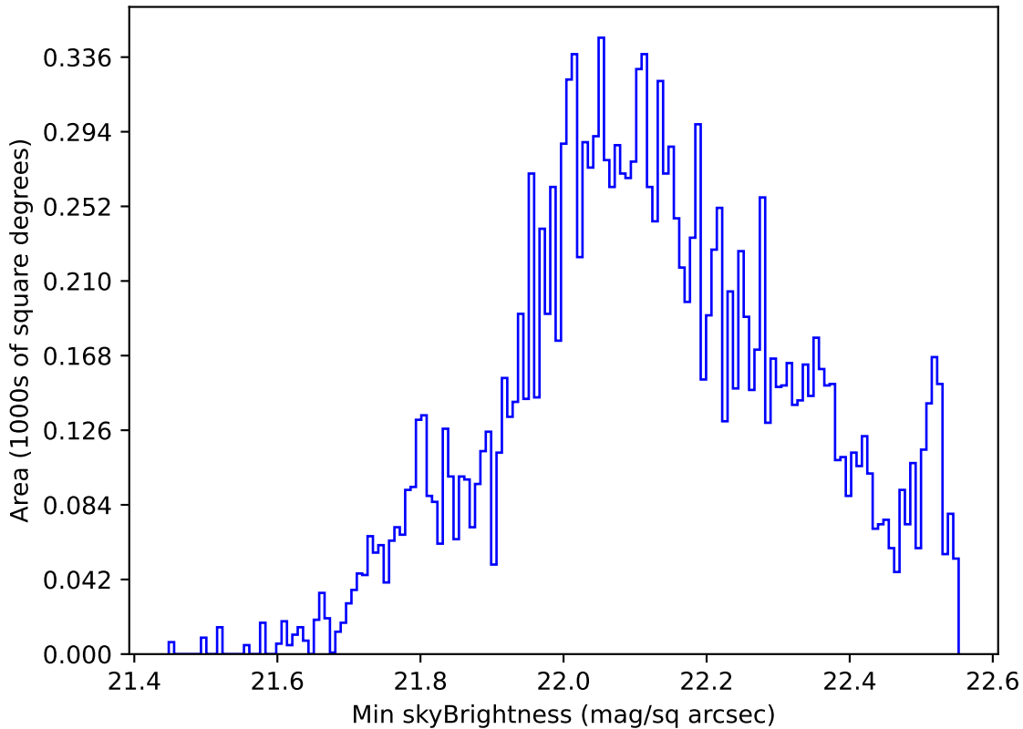
too_elab_r32_d2_ugrizy_v3.4_10yrs WFD u band: Min skyBrightness
