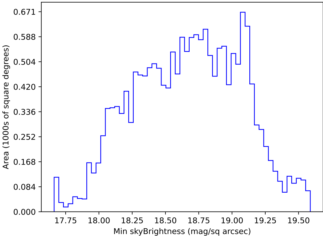
too_elab_r32_d2_ugrizy_v3.4_10yrs WFD r band: Min skyBrightness
