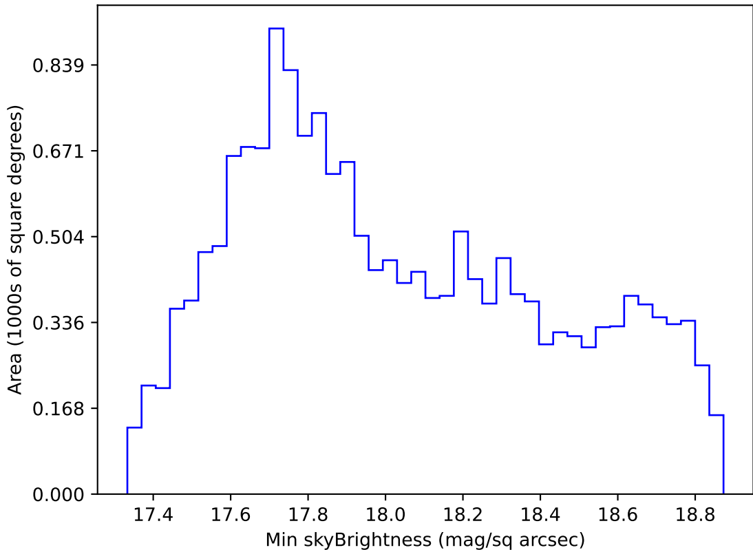
too_elab_r32_d2_ugrizy_v3.4_10yrs WFD i band: Min skyBrightness
