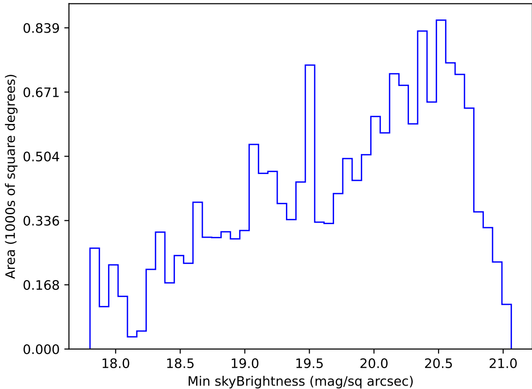
too_elab_r32_d2_ugrizy_v3.4_10yrs WFD g band: Min skyBrightness
