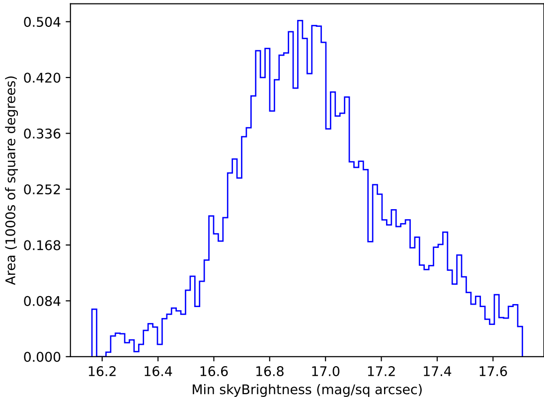
too_elab_r32_d2_ugrizy_v3.4_10yrs WFD all bands: Min skyBrightness
