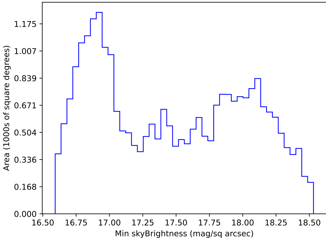
too_elab_r32_d2_ugrizy_v3.4_10yrs All sky z band: Min skyBrightness
