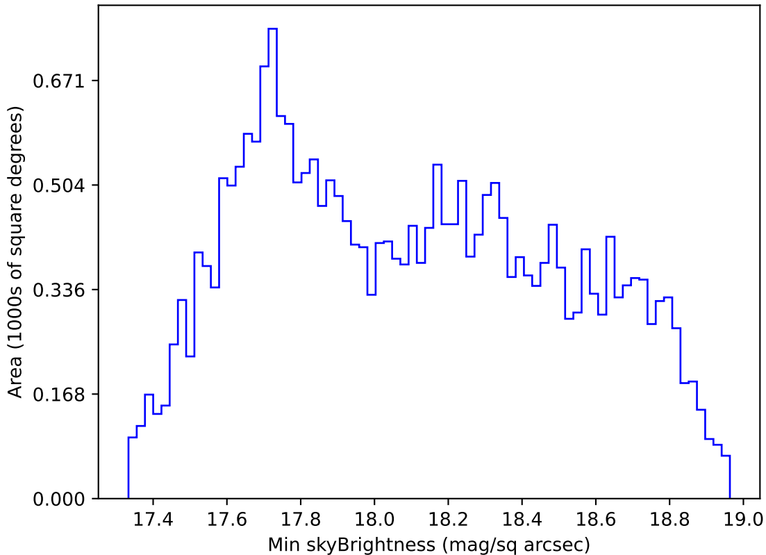
too_elab_r32_d2_ugrizy_v3.4_10yrs All sky i band: Min skyBrightness
