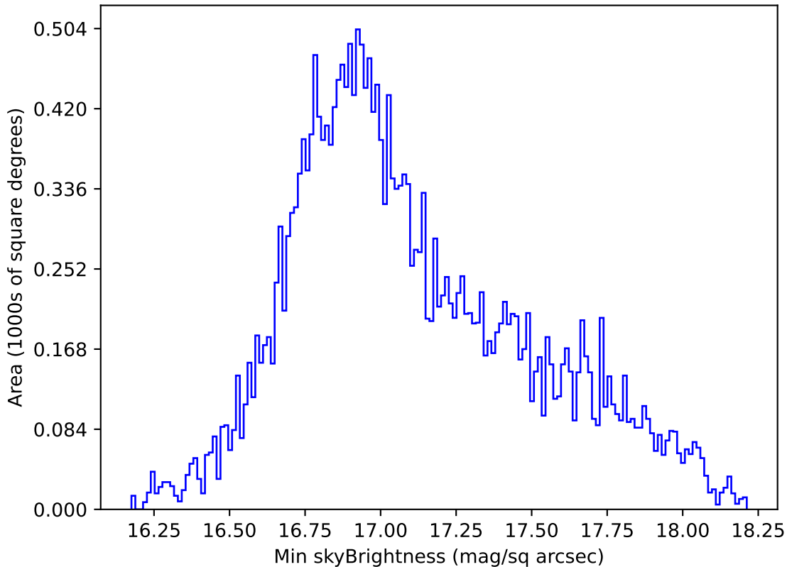
too_elab_r32_d2_ugrizy_v3.4_10yrs All sky all bands: Min skyBrightness
