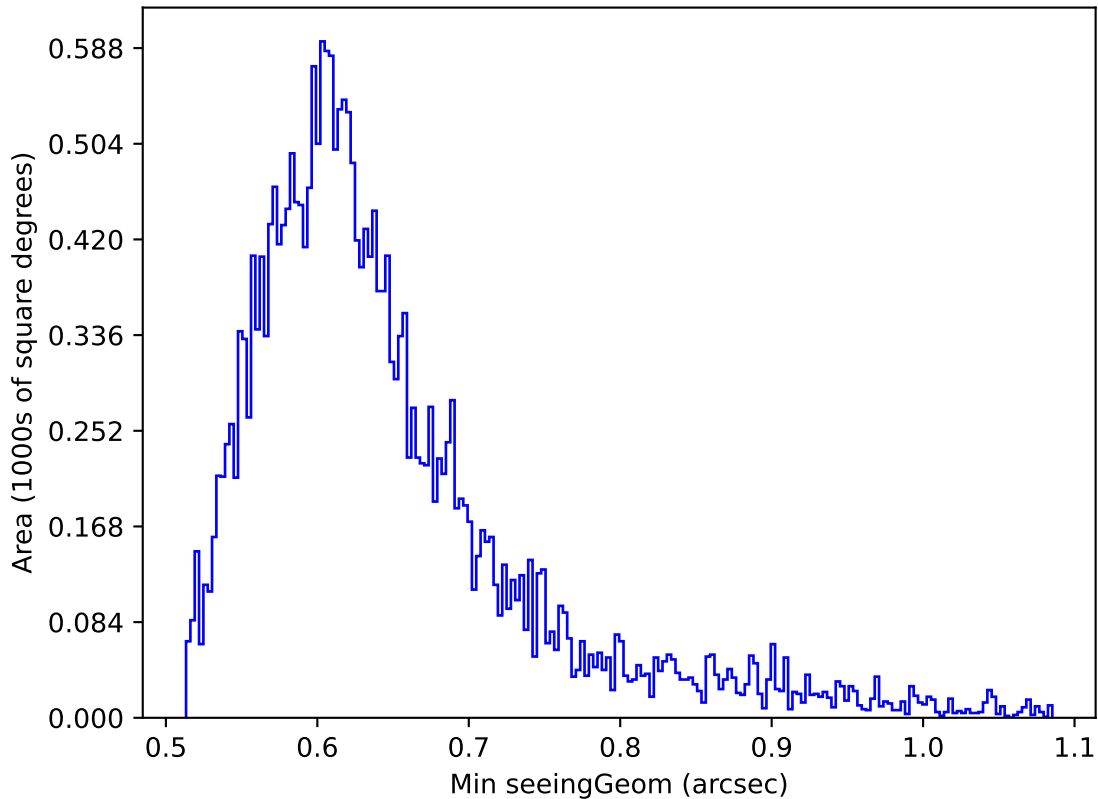
too_elab_r32_d2_ugrizy_v3.4_10yrs Yr 1 z band: Min seeingGeom
