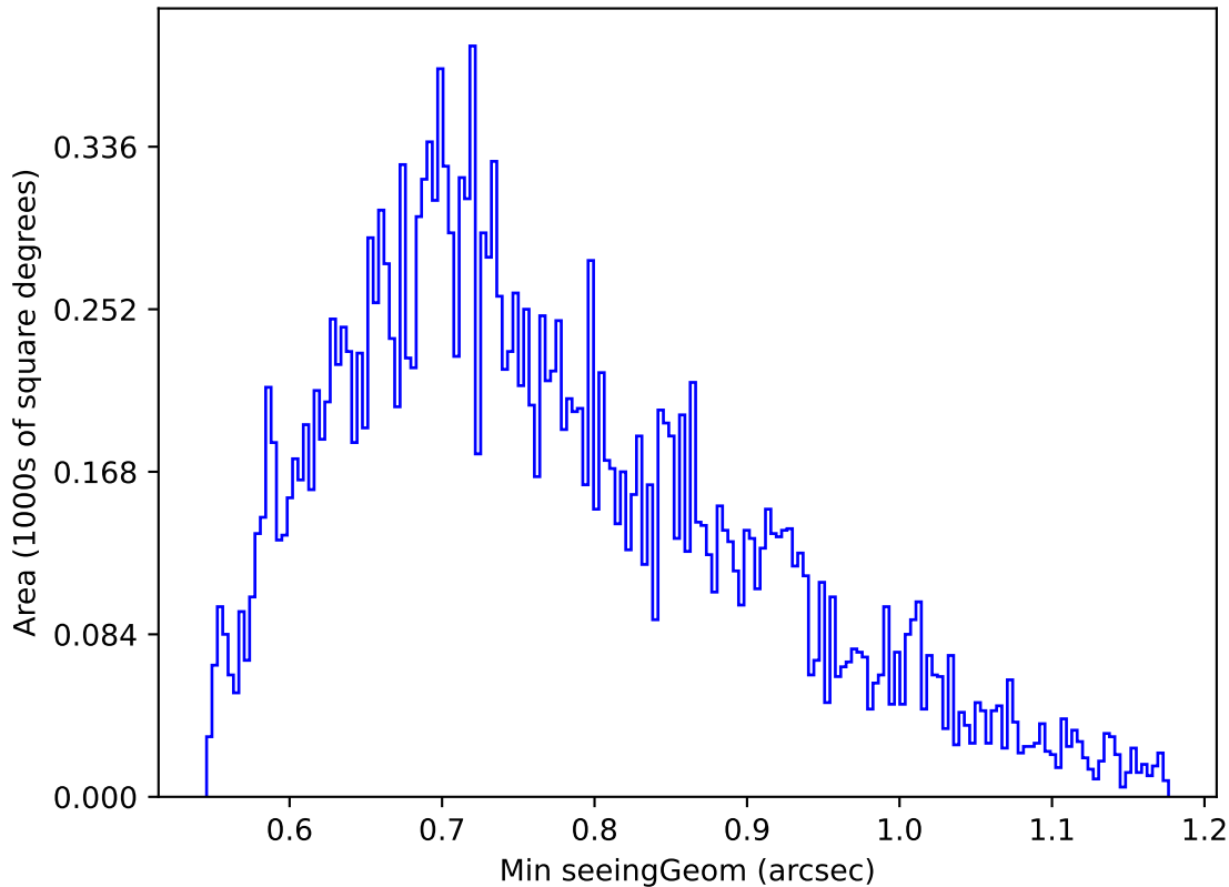
too_elab_r32_d2_ugrizy_v3.4_10yrs Yr 1 u band: Min seeingGeom
