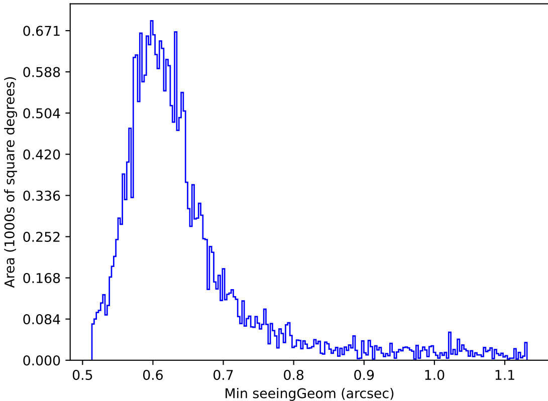
too_elab_r32_d2_ugrizy_v3.4_10yrs Yr 1 r band: Min seeingGeom
