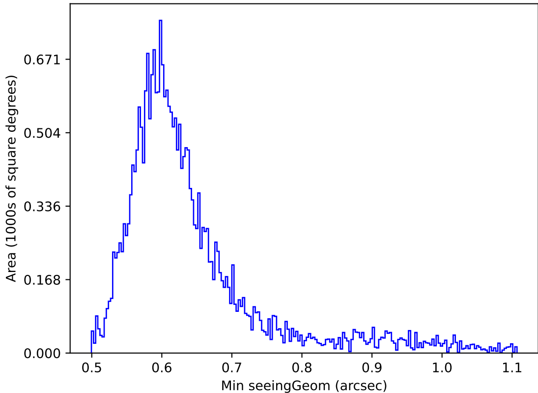
too_elab_r32_d2_ugrizy_v3.4_10yrs Yr 1 i band: Min seeingGeom
