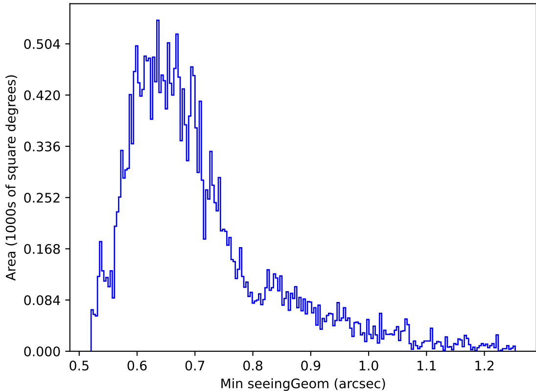
too_elab_r32_d2_ugrizy_v3.4_10yrs Yr 1 g band: Min seeingGeom
