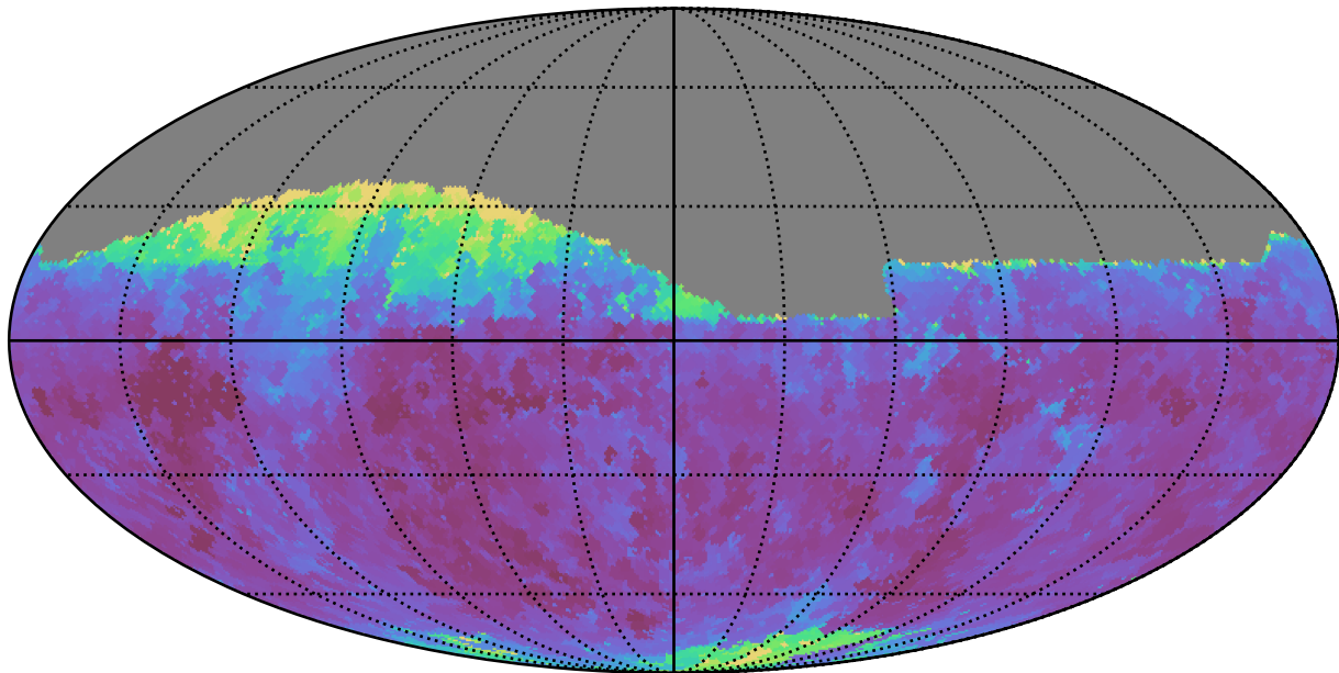
too_elab_r32_d2_ugrizy_v3.4_10yrs Yr 1 i band: Min seeingEff
