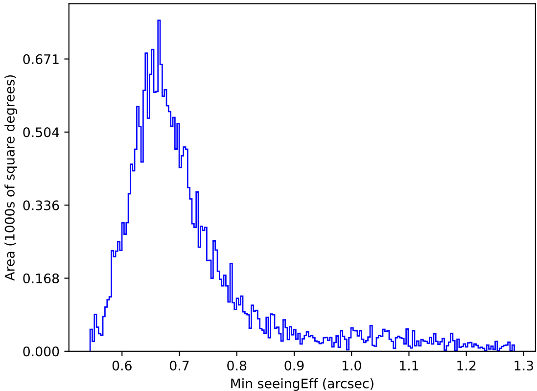
too_elab_r32_d2_ugrizy_v3.4_10yrs Yr 1 i band: Min seeingEff
