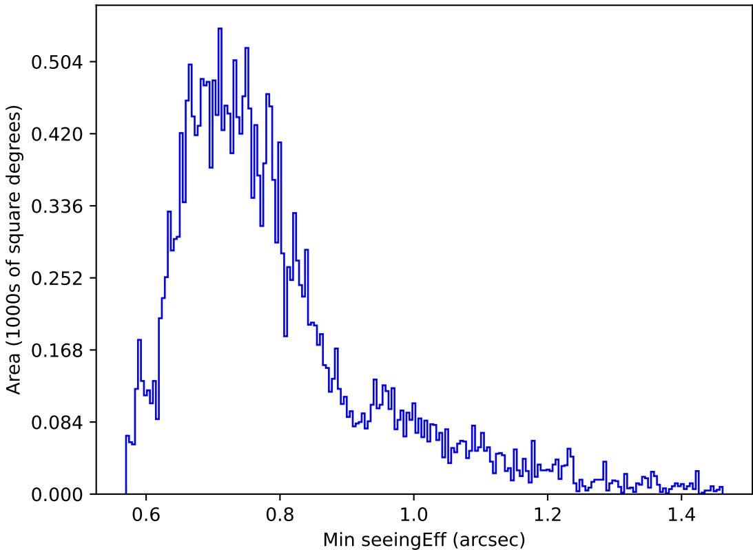
too_elab_r32_d2_ugrizy_v3.4_10yrs Yr 1 g band: Min seeingEff
